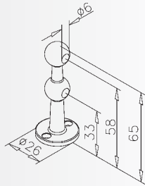
Double mini-fiddle rail centre bracket Doppelte offene Stütze Double support traversant Dubbele opschuifsteun
