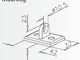
Wall plate Wandauge Oeilleton mural Muuroog
