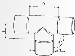
Flush tee Rohrverbinder T Raccord en T T-fitting
