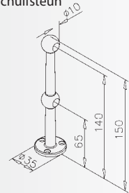
Double fiddle rail centre bracket Doppelte offene Stütze Double support traversant Dubbele opschuifsteun
