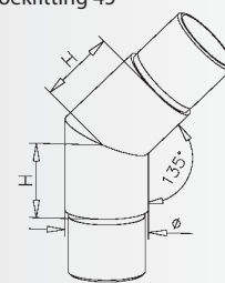
Flush angle 45° Rohrverbinder 45° Raccord 45° Hoekfitting 45°
