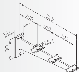
Tray slide bracket Tablettruscenträger Support porte-plateaux Buizensteun
