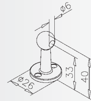
Mini-fiddle rail centre bracket Offene Stütze Support traversant Opschuifsteun
